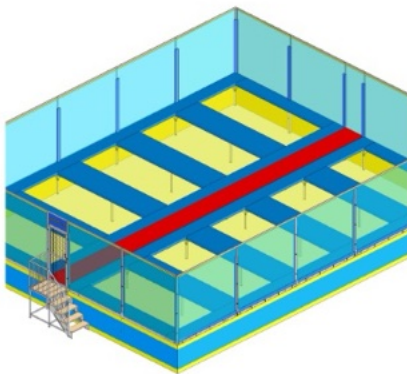
ART. 110.1 - trampoline 10 standard seats in two lines, central corridor
